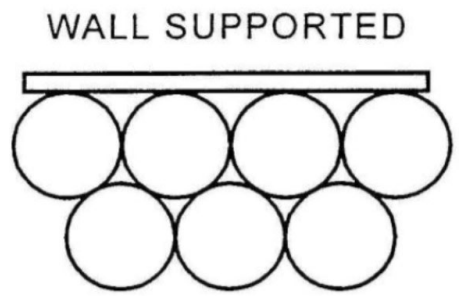
Correct Nesting (contact on 3 Points)
